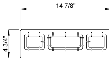
4 INSERT - TOP VIEW 1 1/2" = 1'-0"
