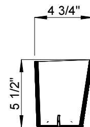
5 INSERT - SIDE VIEW 1 1/2" = 1'-0"
