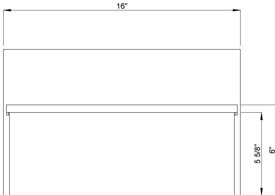
1 FRONT VIEW 3" = 1'-0"
