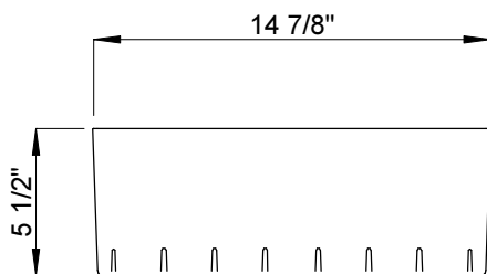
3 INSERT - FRONT VIEW 1 1/2" = 1'-0"
