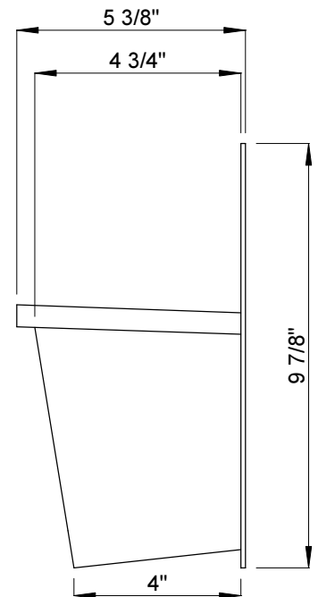
2 SIDE VIEW 3" = 1'-0"
