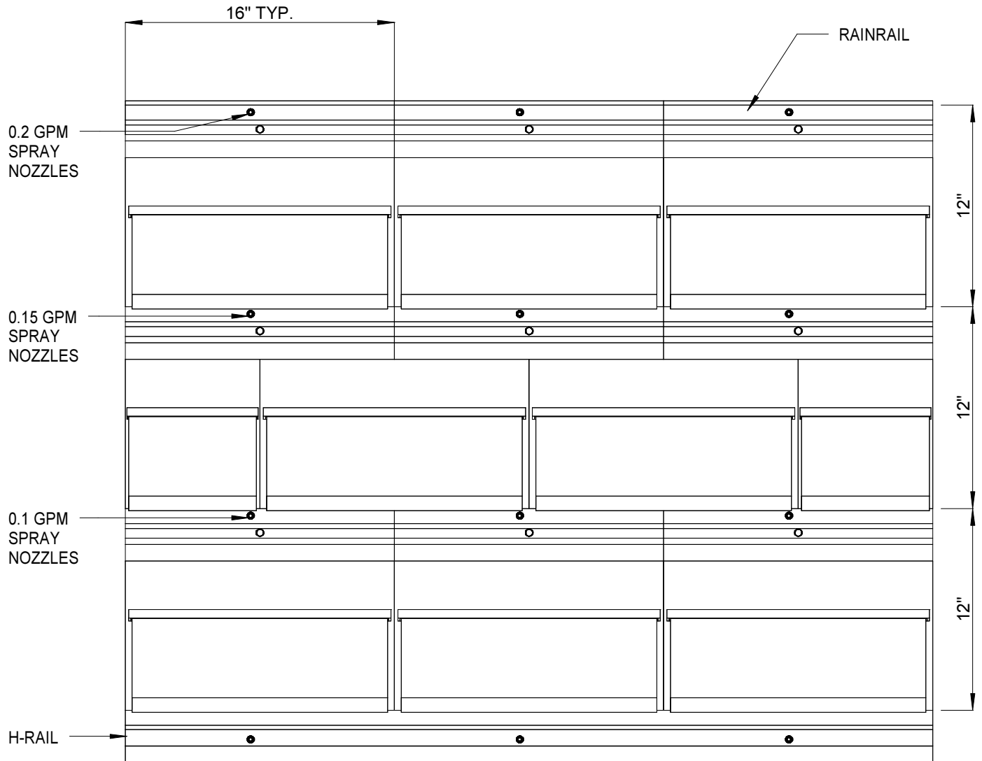
1 EXTERIOR WALL APPLICATION-FRONT VIEW 1 1/2" = 1'-0"
