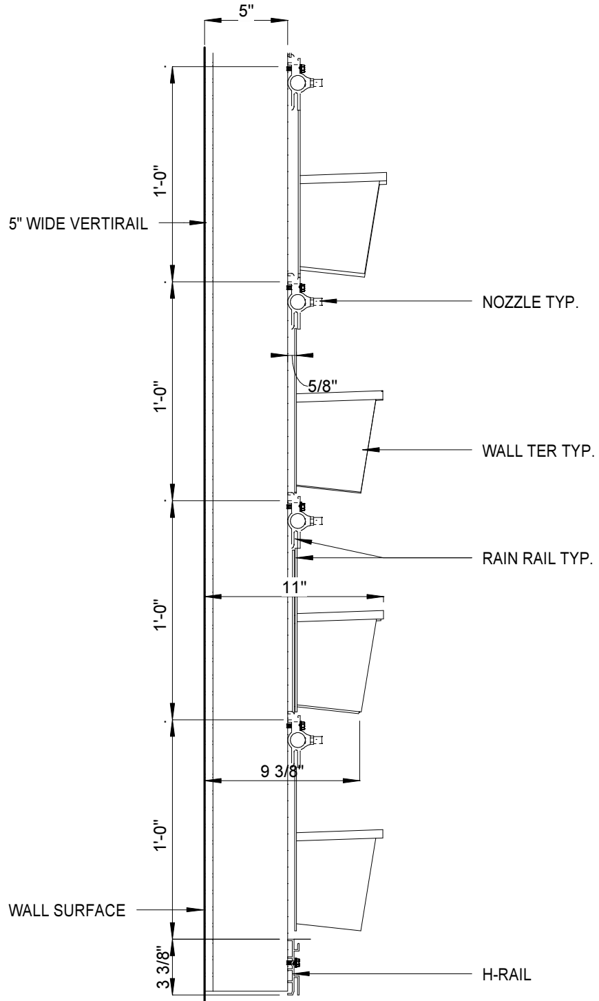
1 EXTERIOR WALL APPLICATION SECTION WITH REAR TAP IRRIGATION 1 1/2" = 1'-0"
