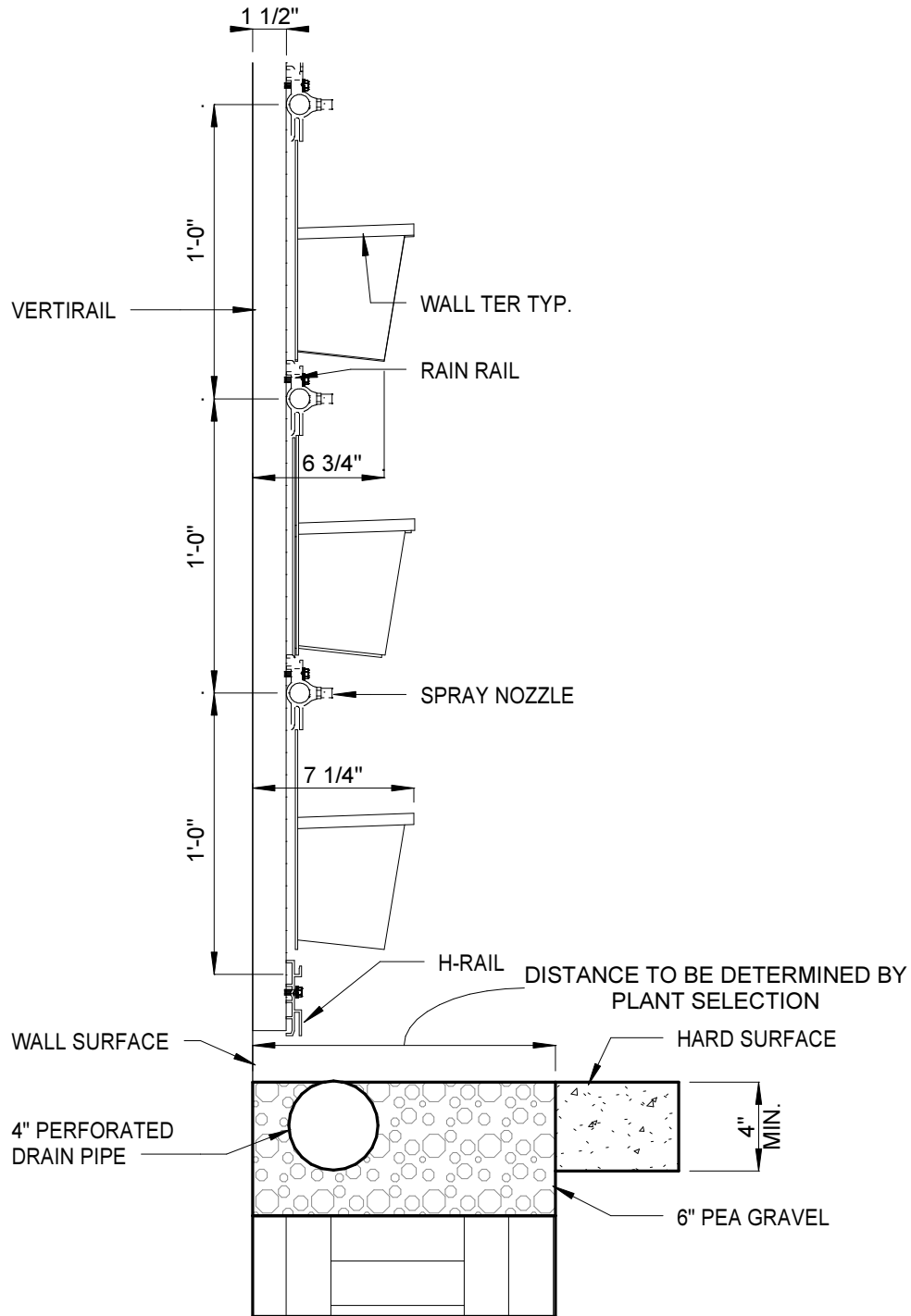
1 EXTERIOR APPLICATION WALL SECTION 1 1/2" = 1'-0"
